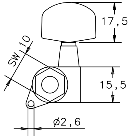
linke Mechanik left machine head
