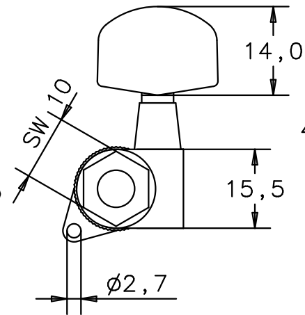
linke Mechanik left machine head
